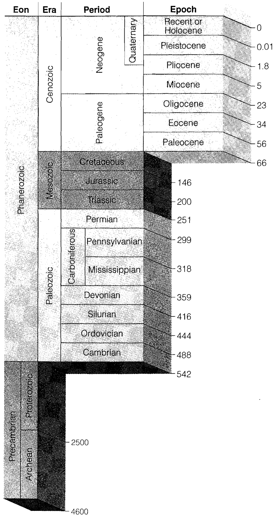
Figure 1.17 The Geologic Time Scale The numbers to the right of the columns are ages in millions of years before the present. Dates are from Gradstein, F., J. Ogg and A. Smith. A Geologic Time Scale 2004 (Cambridge, UK: Cambridge University Press, 2005), Figure 1.2
