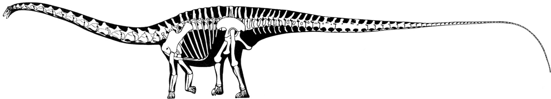
Figure 20.11. Skeletal reconstruction of Diplodocus . Femur length 1542 mm.
